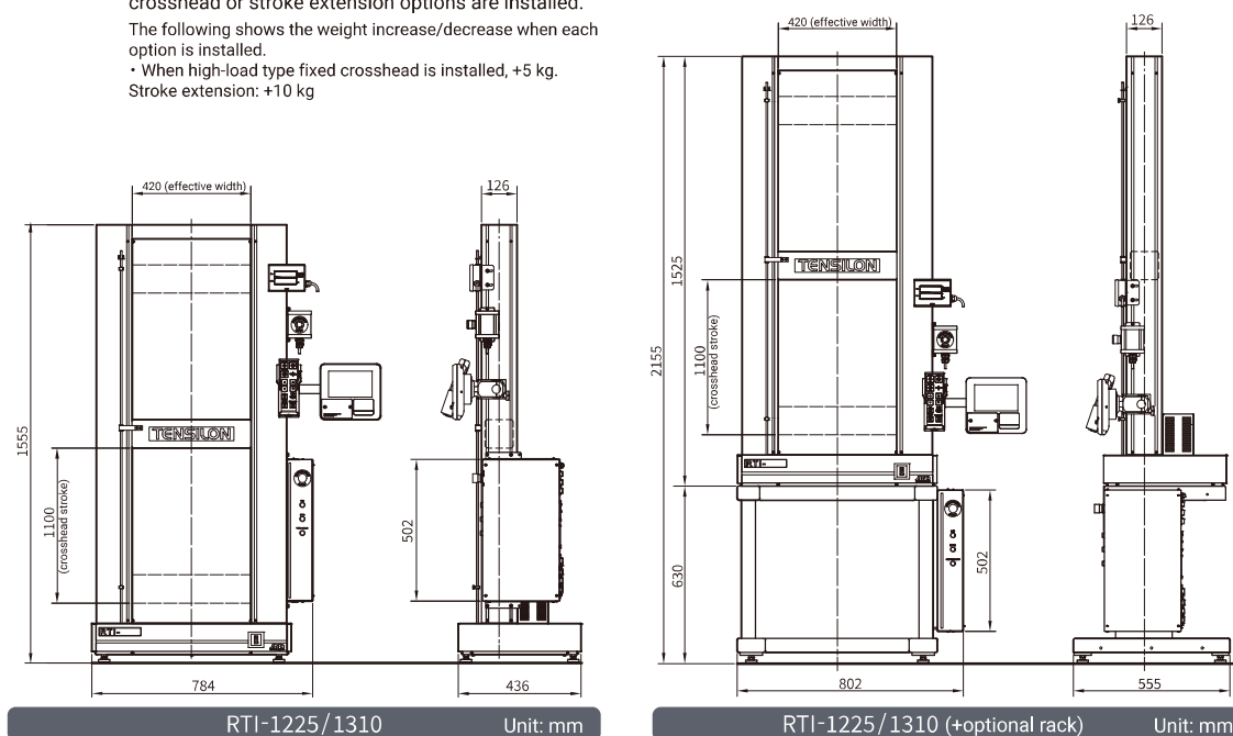
RTI-1225/1310 (+optional rack)
